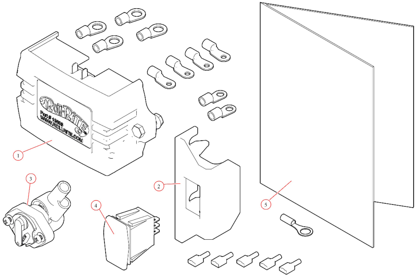
10914 Electric Kit, With 10698 Relay and Rocker Switch
